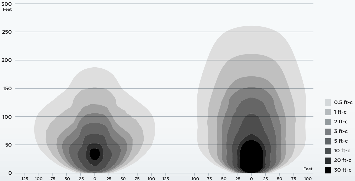
Night-Lite™ V-Series* with 4 - 320 W Conssin LED Light Output Area Lit to .5 Foot Candle (ft-c) or Higher: 28,449 ft 2
